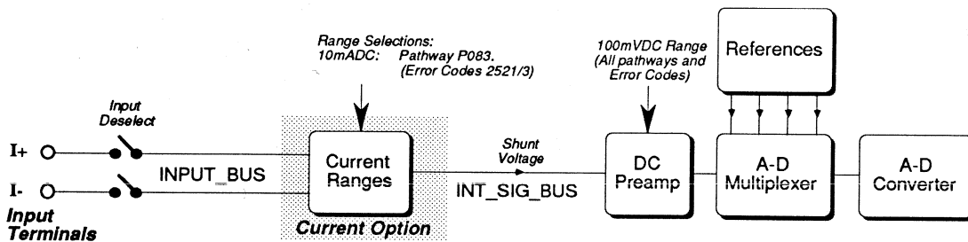
DC Current. 2.6.9: 10mA Range - Zero Checks - Simplified Test Setup Diagram
